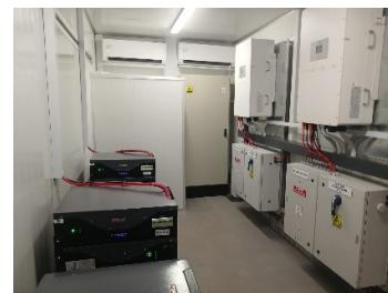
150KW-HYBRID-SYSTEM-CURRO-KATHU
